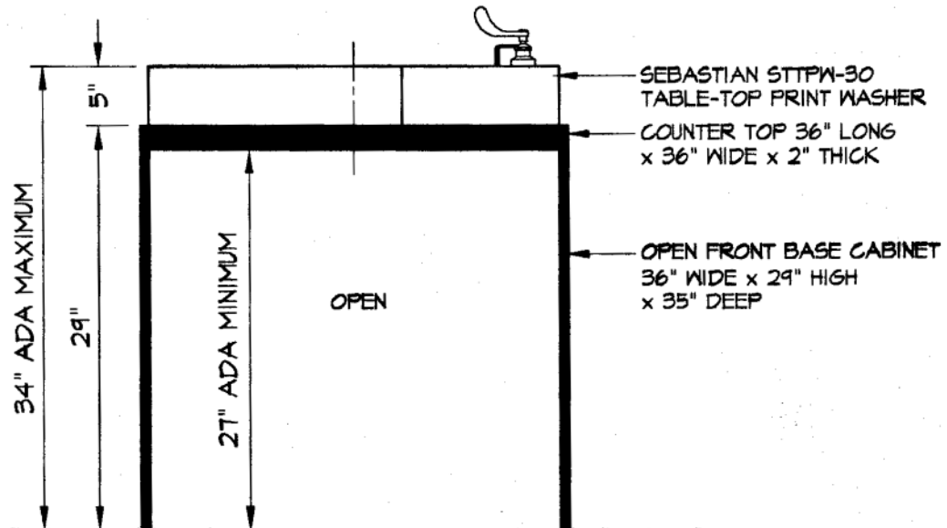
SEBASTIAN STTPW-30 TABLE TOP WASHER MOUNTED ON AN OPEN CABINET
